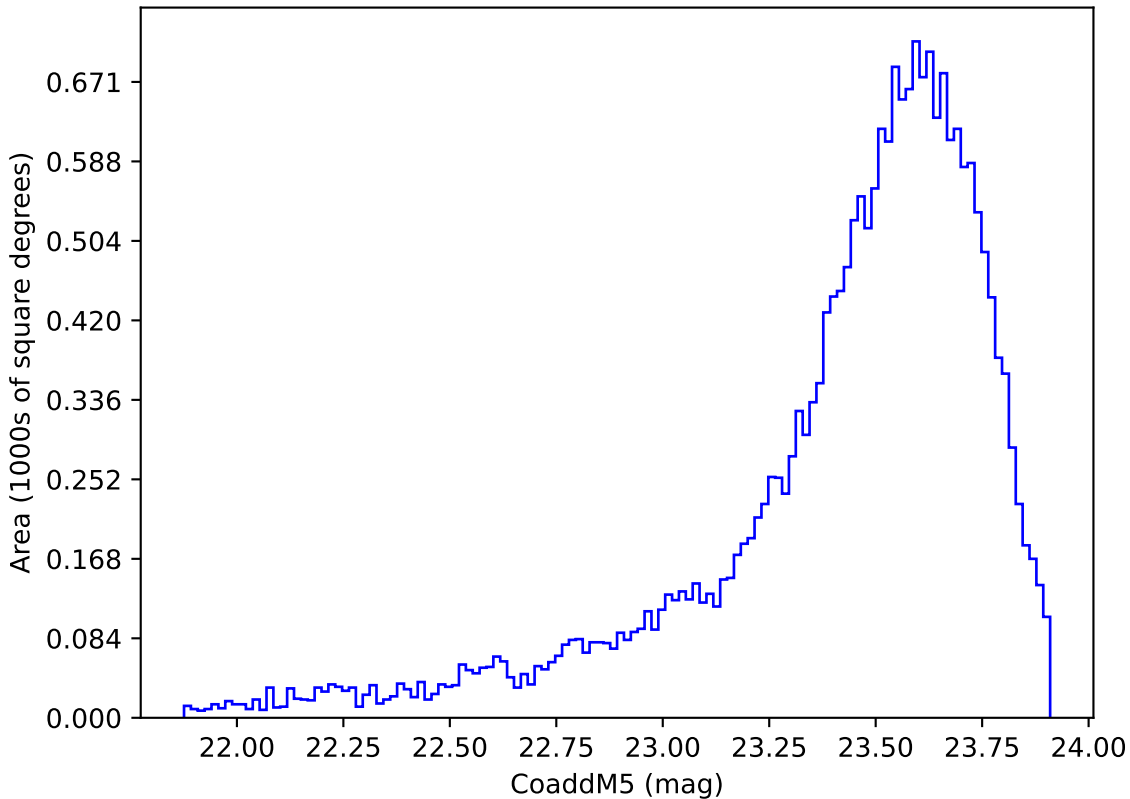
noroll_mjdp60_v3.4_10yrs Yr 3-4 y band: CoaddM5
