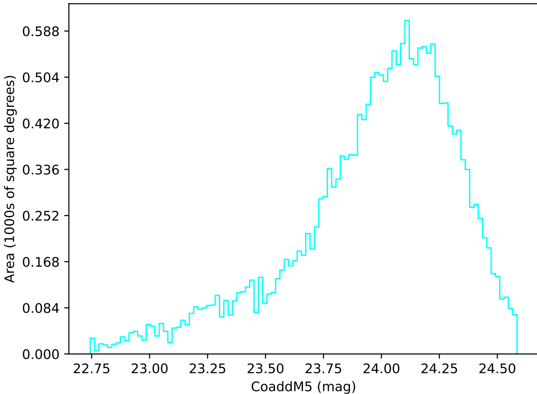
noroll_mjdp60_v3.4_10yrs Yr 3-4 u band: CoaddM5
