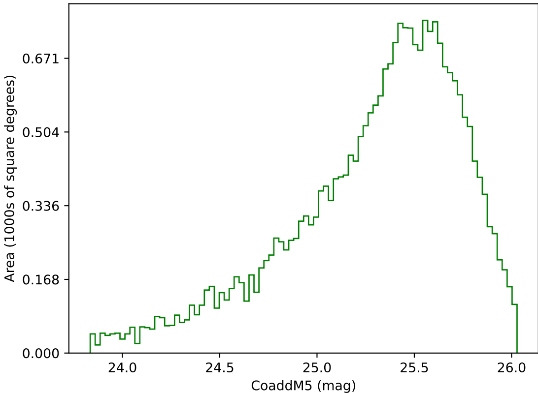
noroll_mjdp60_v3.4_10yrs Yr 3-4 g band: CoaddM5
