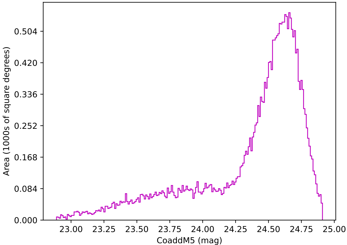
noroll_mjdp60_v3.4_10yrs Yr 1 z band: CoaddM5
