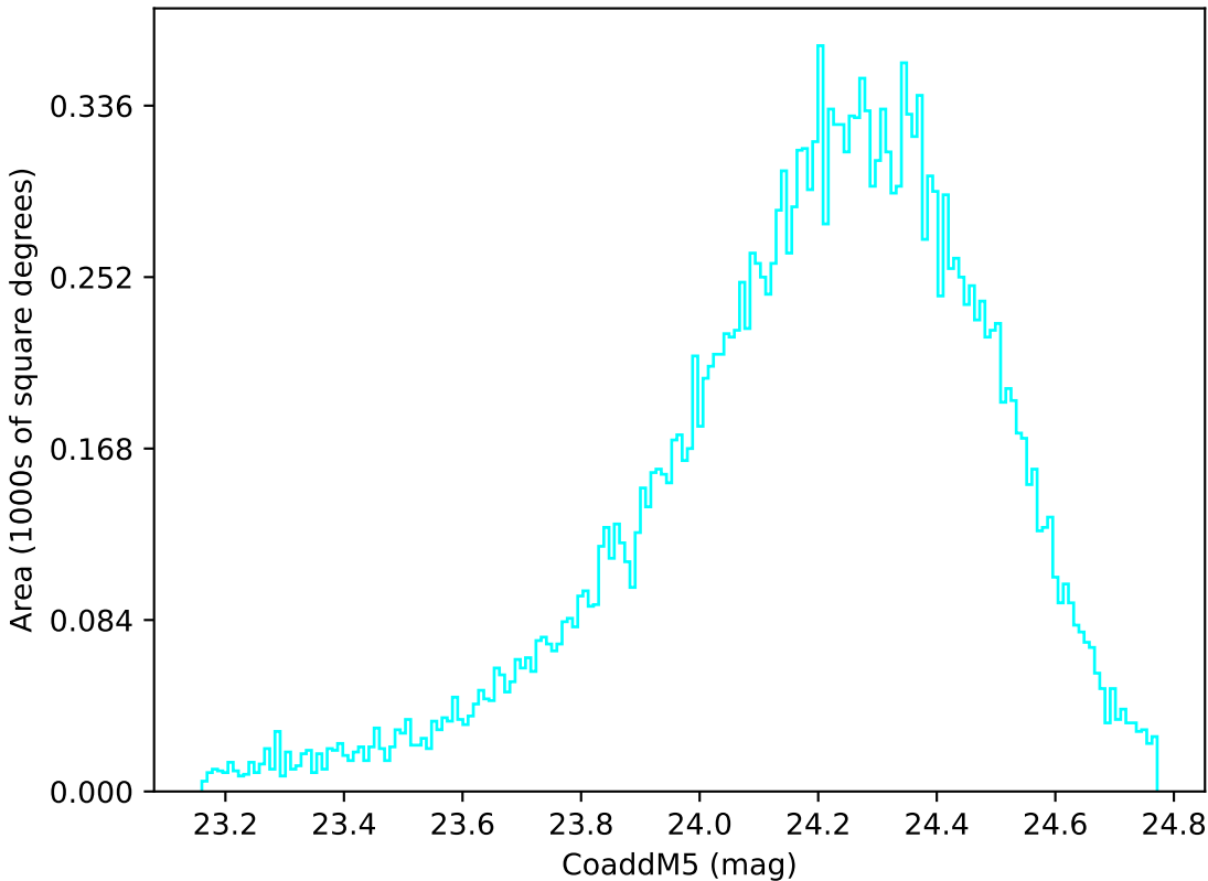
noroll_mjdp60_v3.4_10yrs Yr 1 u band: CoaddM5
