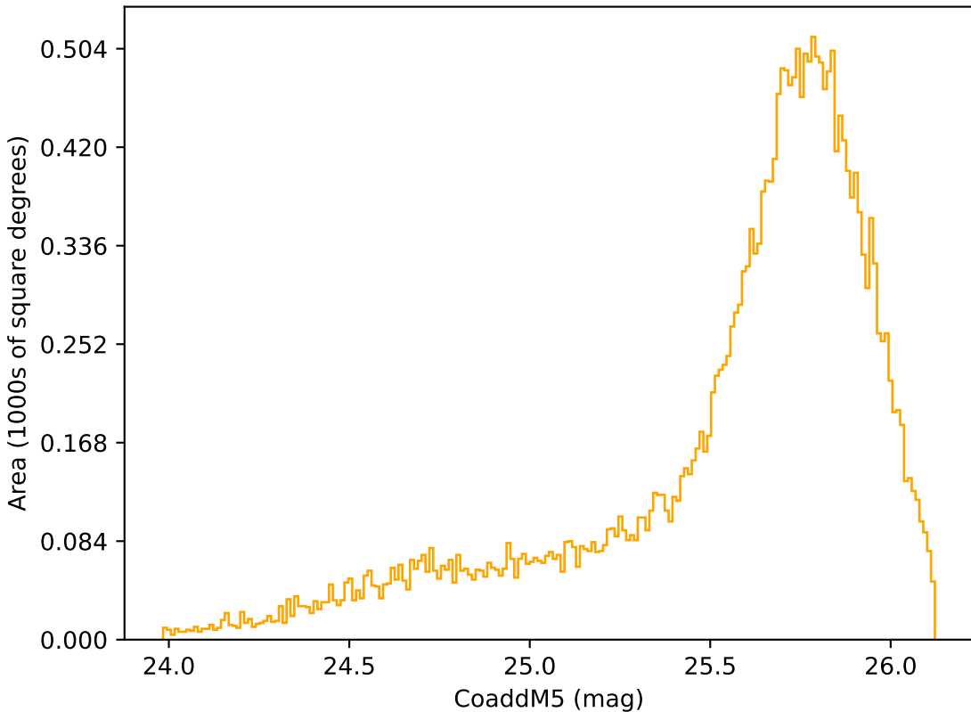
noroll_mjdp60_v3.4_10yrs Yr 1 r band: CoaddM5
