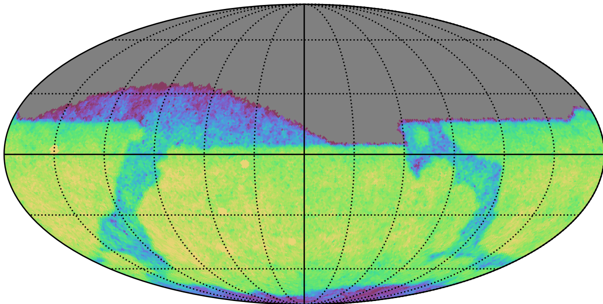
noroll_mjdp60_v3.4_10yrs Yr 1 i band: CoaddM5
