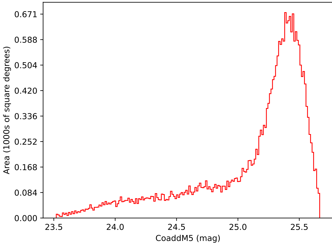
noroll_mjdp60_v3.4_10yrs Yr 1 i band: CoaddM5
