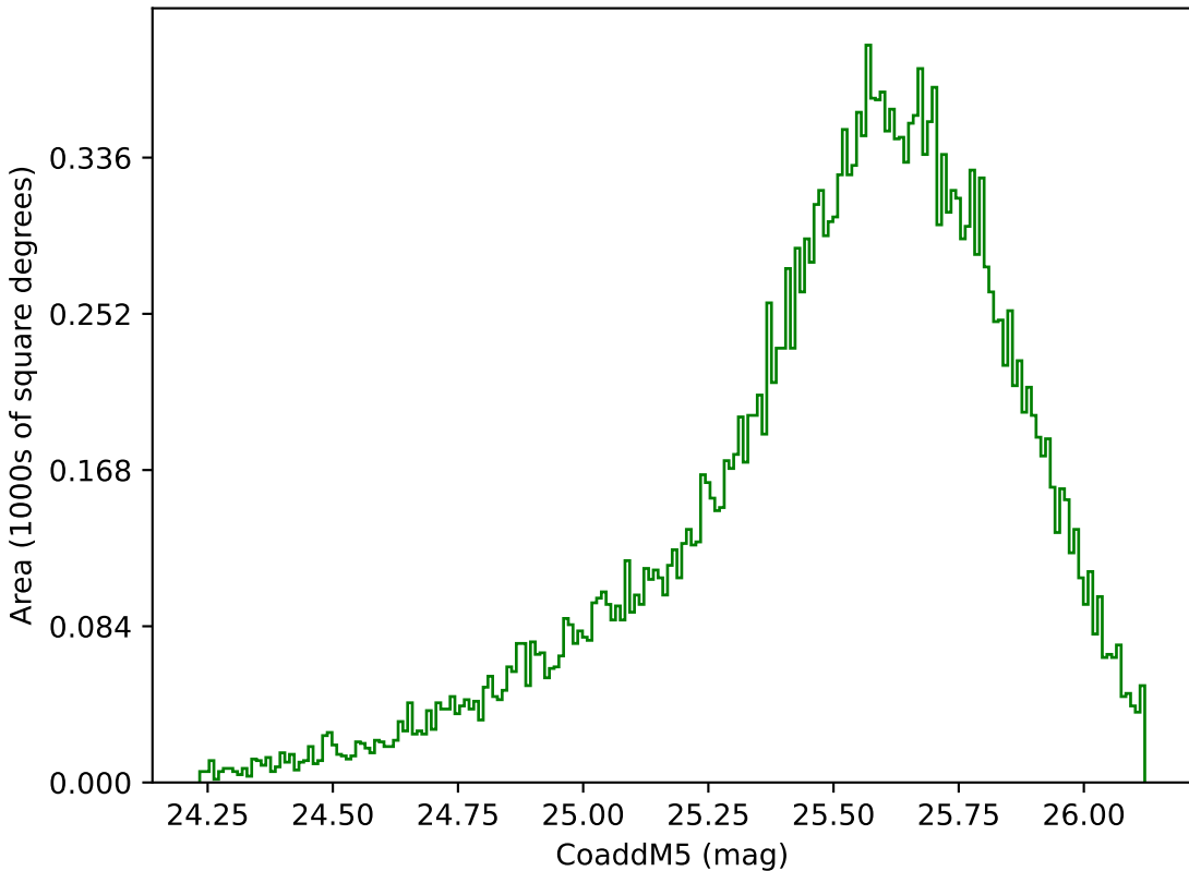
noroll_mjdp60_v3.4_10yrs Yr 1 g band: CoaddM5
