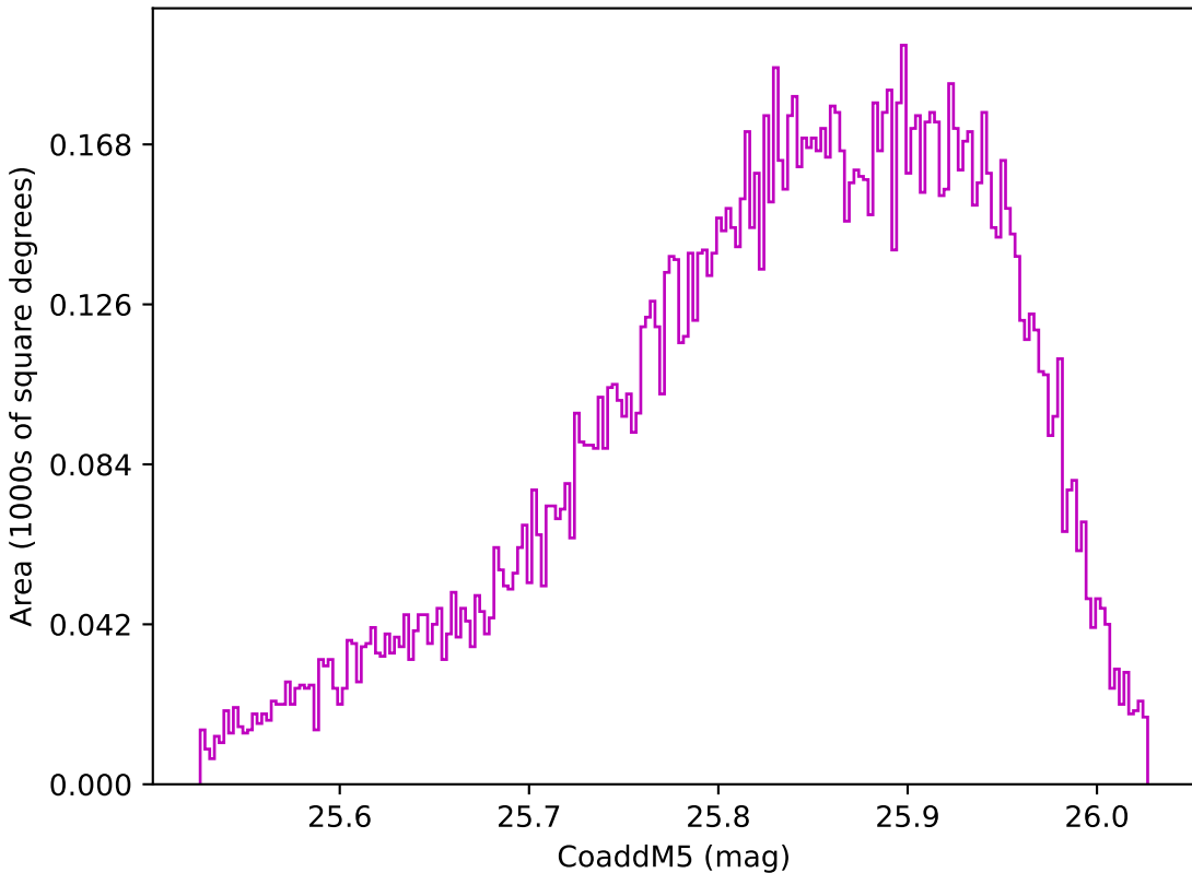
noroll_mjdp60_v3.4_10yrs WFD z band: CoaddM5
