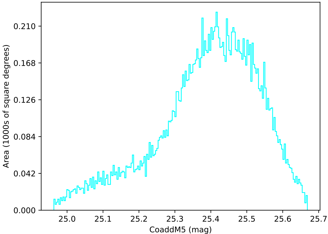
noroll_mjdp60_v3.4_10yrs WFD u band: CoaddM5
