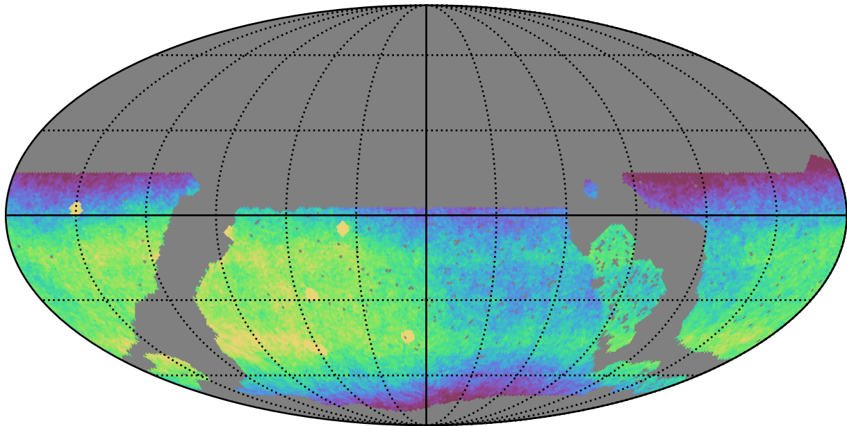
noroll_mjdp60_v3.4_10yrs WFD r band: CoaddM5
