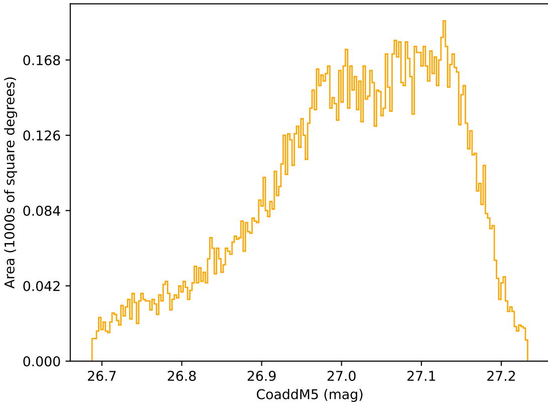
noroll_mjdp60_v3.4_10yrs WFD r band: CoaddM5
