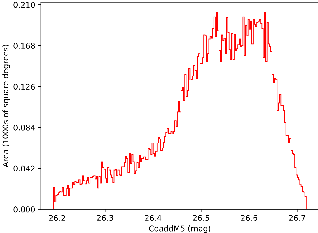
noroll_mjdp60_v3.4_10yrs WFD i band: CoaddM5
