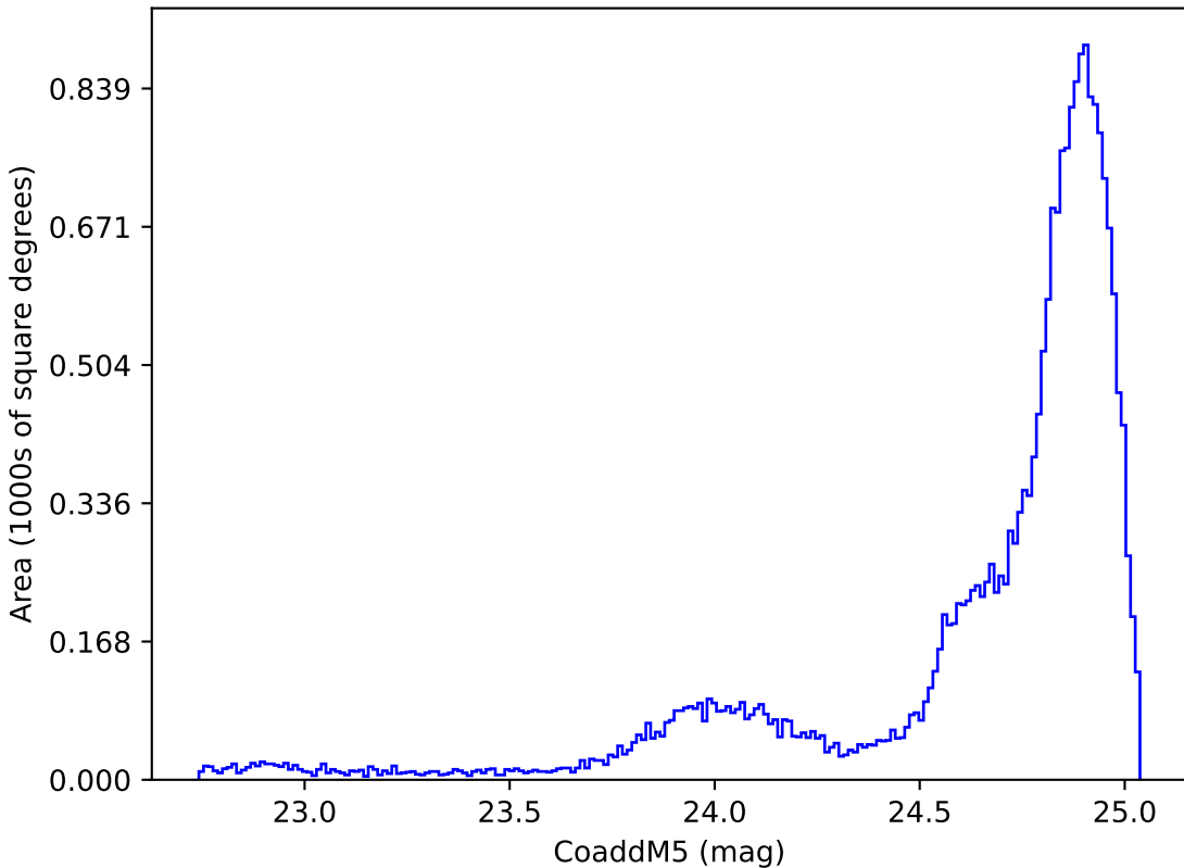
noroll_mjdp60_v3.4_10yrs All sky y band: CoaddM5
