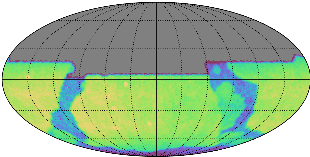
noroll_mjdp60_v3.4_10yrs All sky u band: CoaddM5
