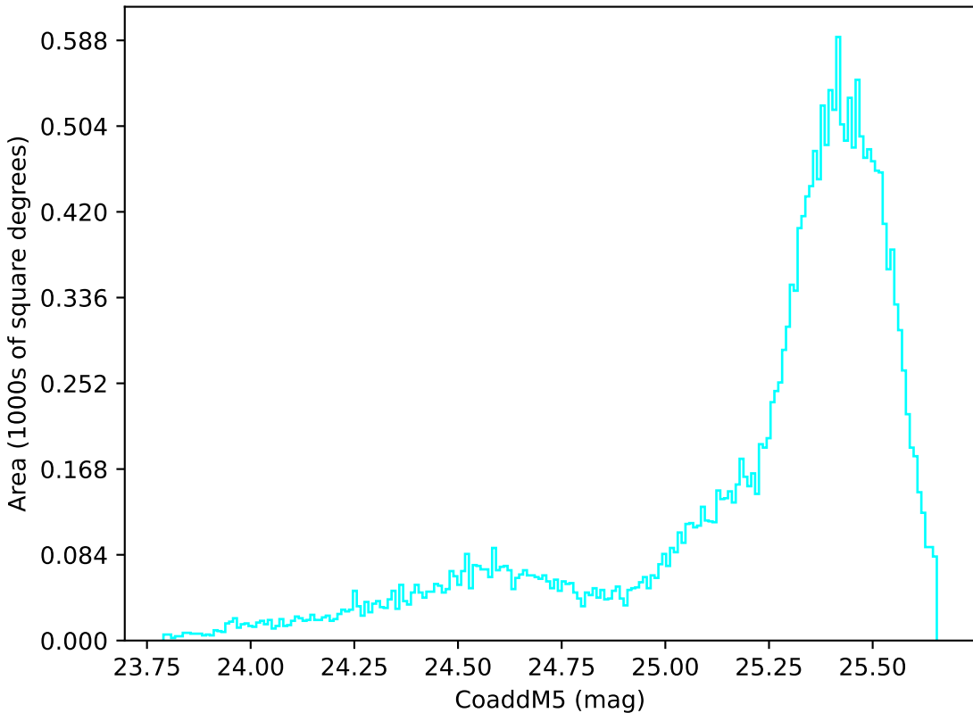
noroll_mjdp60_v3.4_10yrs All sky u band: CoaddM5
