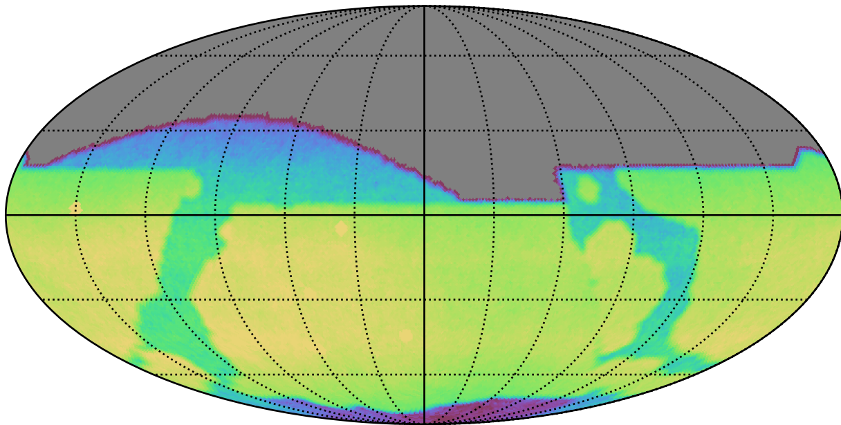
noroll_mjdp60_v3.4_10yrs All sky r band: CoaddM5
