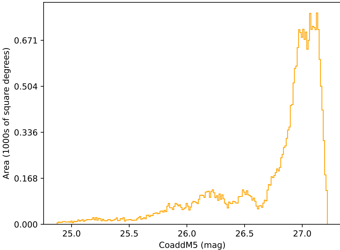
noroll_mjdp60_v3.4_10yrs All sky r band: CoaddM5
