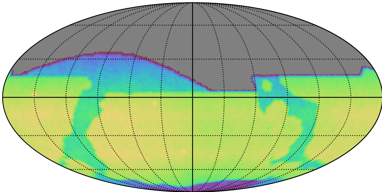
noroll_mjdp60_v3.4_10yrs All sky i band: CoaddM5
