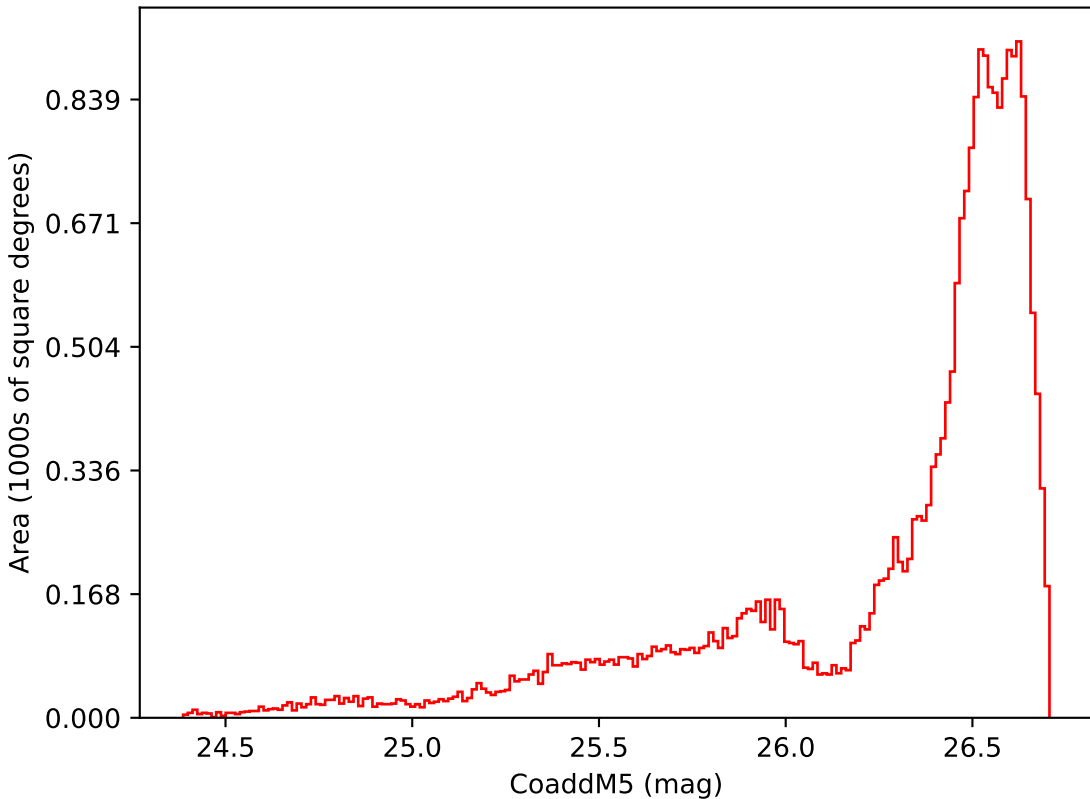
noroll_mjdp60_v3.4_10yrs All sky i band: CoaddM5
