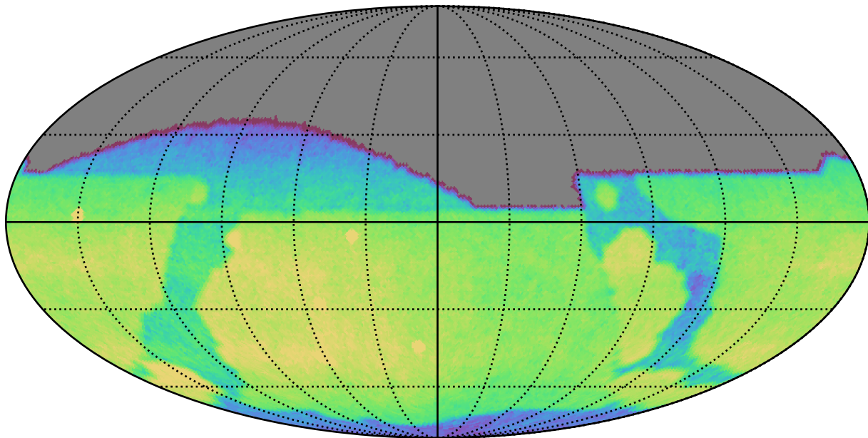
noroll_mjdp60_v3.4_10yrs All sky g band: CoaddM5
