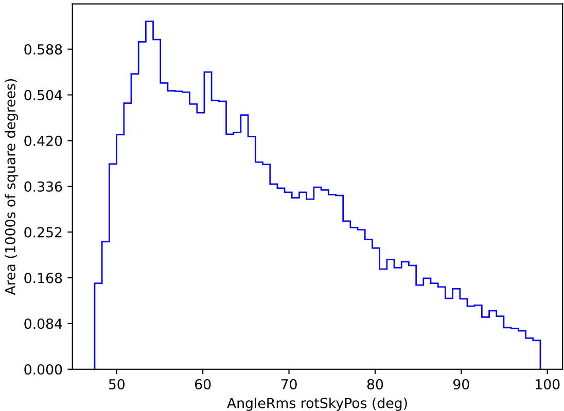
noroll_mjdp60_v3.4_10yrs WFD z band: AngleRms rotSkyPos
