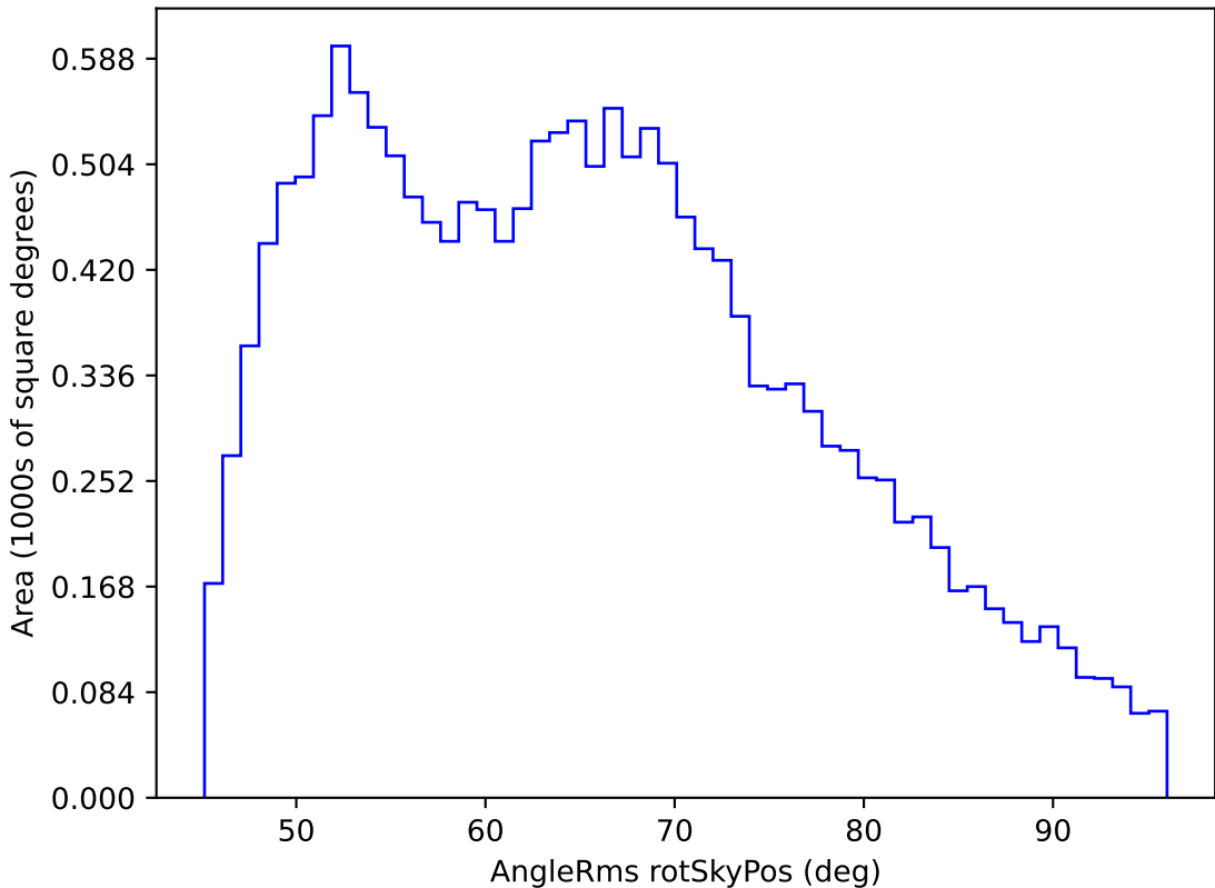
noroll_mjdp60_v3.4_10yrs WFD y band: AngleRms rotSkyPos
