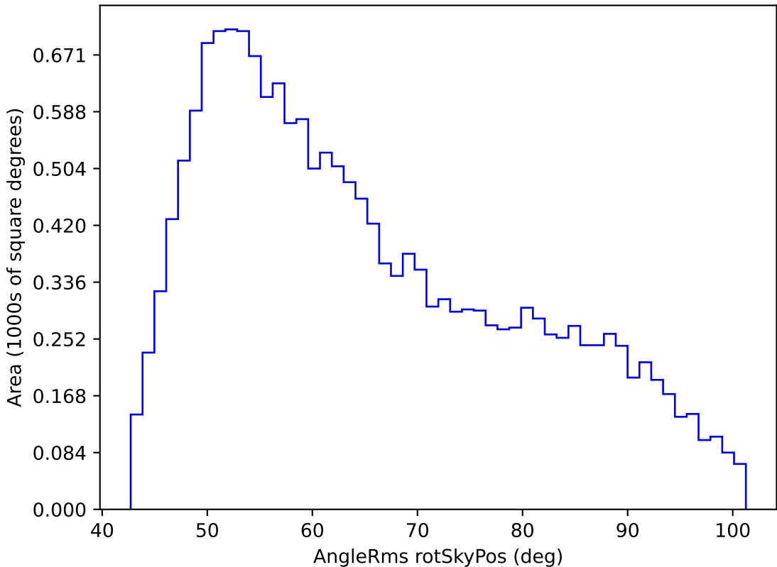
noroll_mjdp60_v3.4_10yrs WFD u band: AngleRms rotSkyPos
