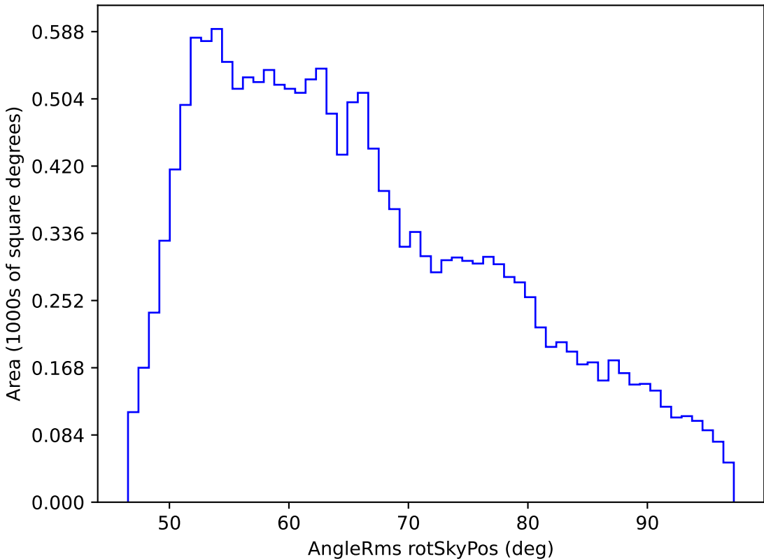
noroll_mjdp60_v3.4_10yrs WFD i band: AngleRms rotSkyPos
