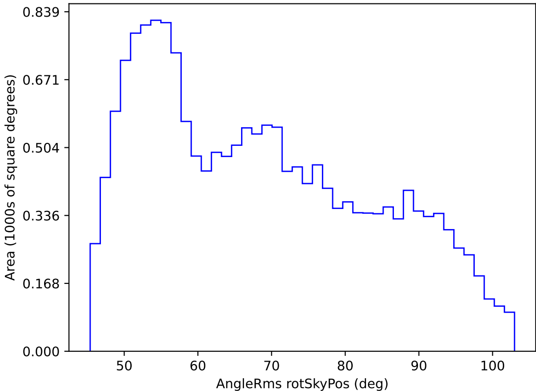
noroll_mjdp60_v3.4_10yrs WFD g band: AngleRms rotSkyPos
