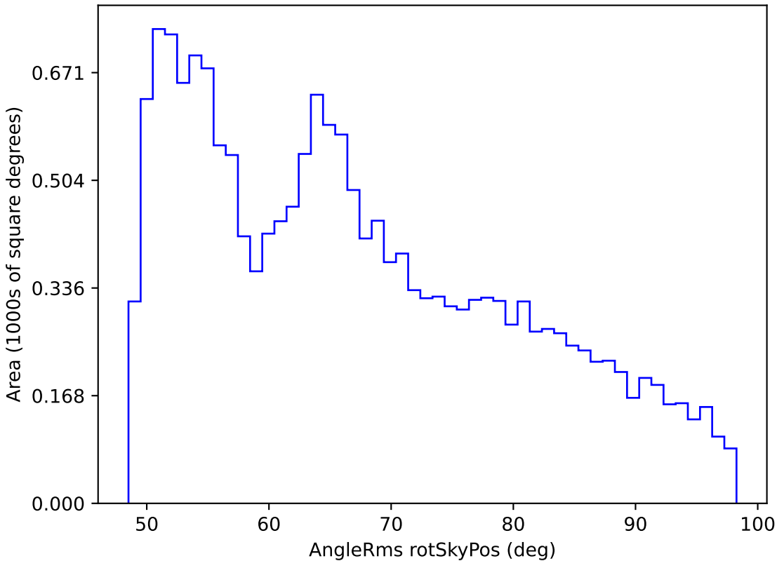
noroll_mjdp60_v3.4_10yrs WFD all bands: AngleRms rotSkyPos
