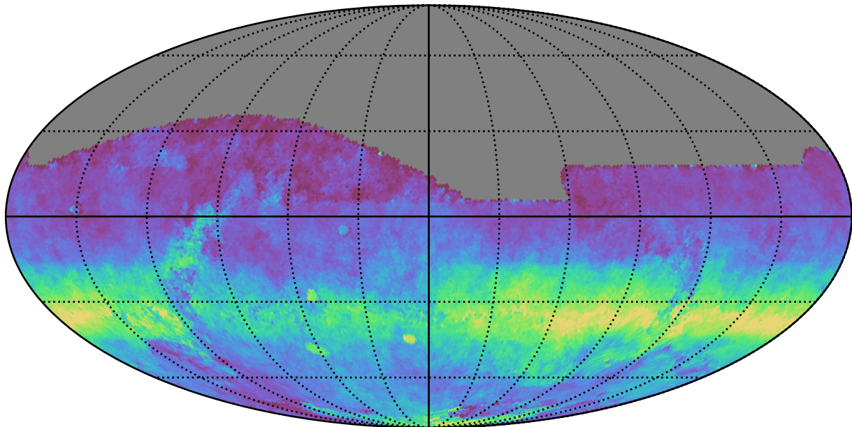
noroll_mjdp60_v3.4_10yrs All sky z band: AngleRms rotSkyPos
