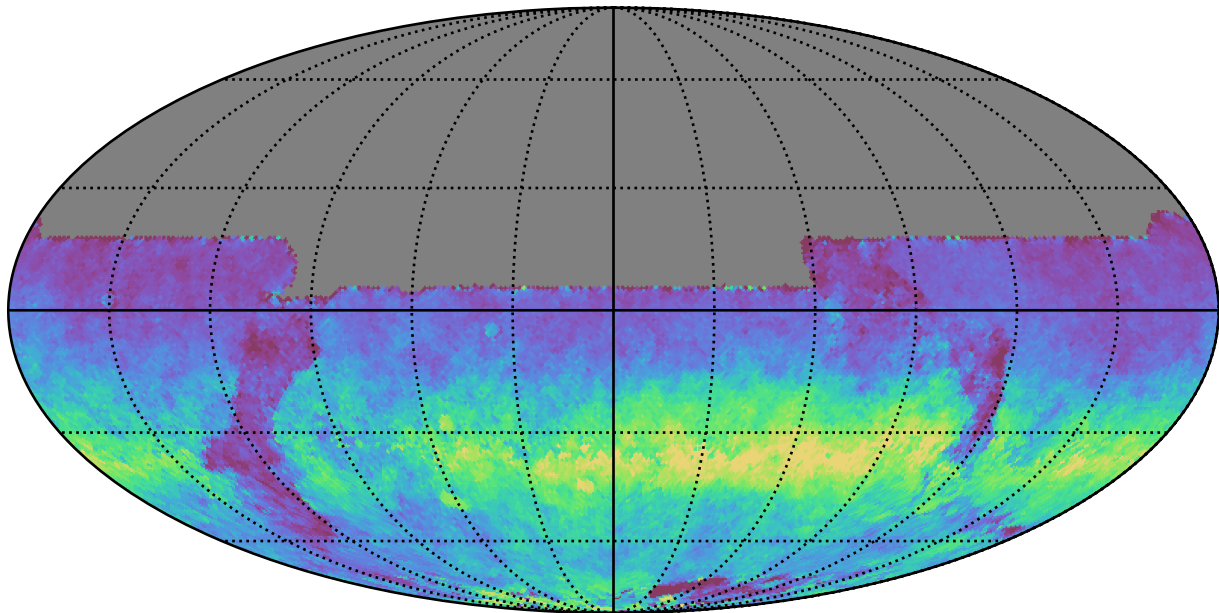
noroll_mjdp60_v3.4_10yrs All sky y band: AngleRms rotSkyPos
