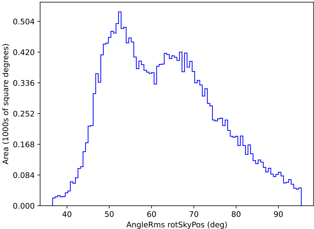
noroll_mjdp60_v3.4_10yrs All sky y band: AngleRms rotSkyPos
