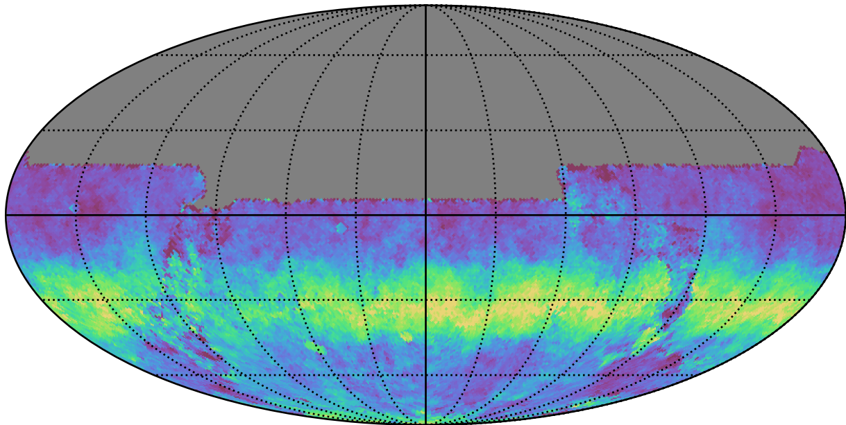
noroll_mjdp60_v3.4_10yrs All sky u band: AngleRms rotSkyPos
