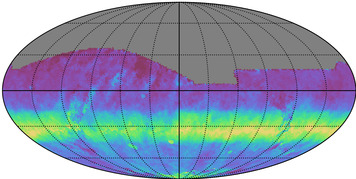
noroll_mjdp60_v3.4_10yrs All sky r band: AngleRms rotSkyPos
