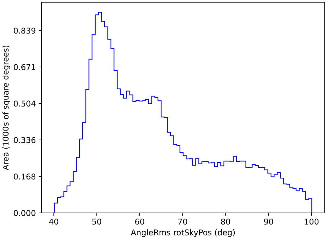
noroll_mjdp60_v3.4_10yrs All sky r band: AngleRms rotSkyPos
