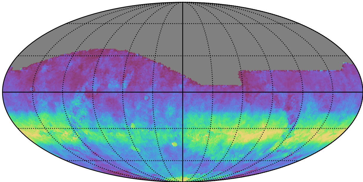
noroll_mjdp60_v3.4_10yrs All sky i band: AngleRms rotSkyPos
