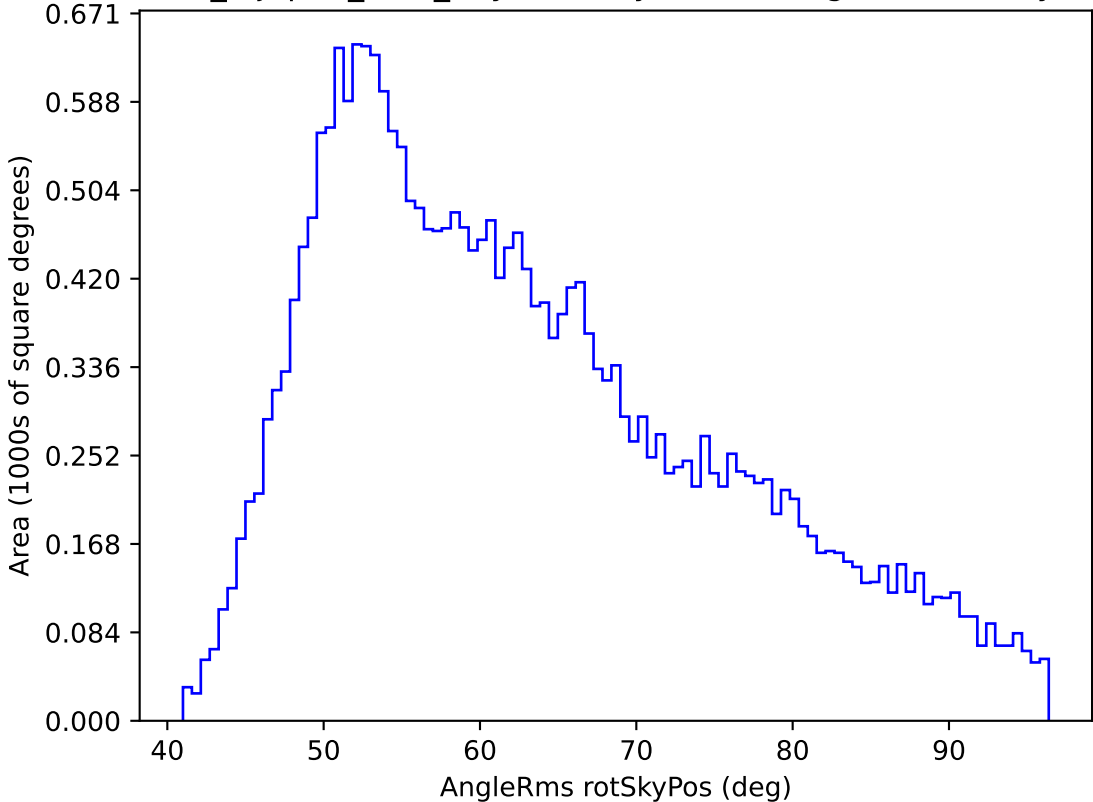
noroll_mjdp60_v3.4_10yrs All sky i band: AngleRms rotSkyPos
