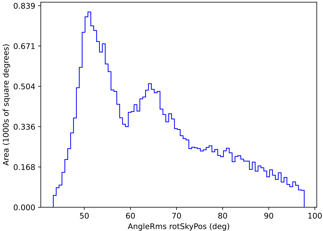
noroll_mjdp60_v3.4_10yrs All sky all bands: AngleRms rotSkyPos
