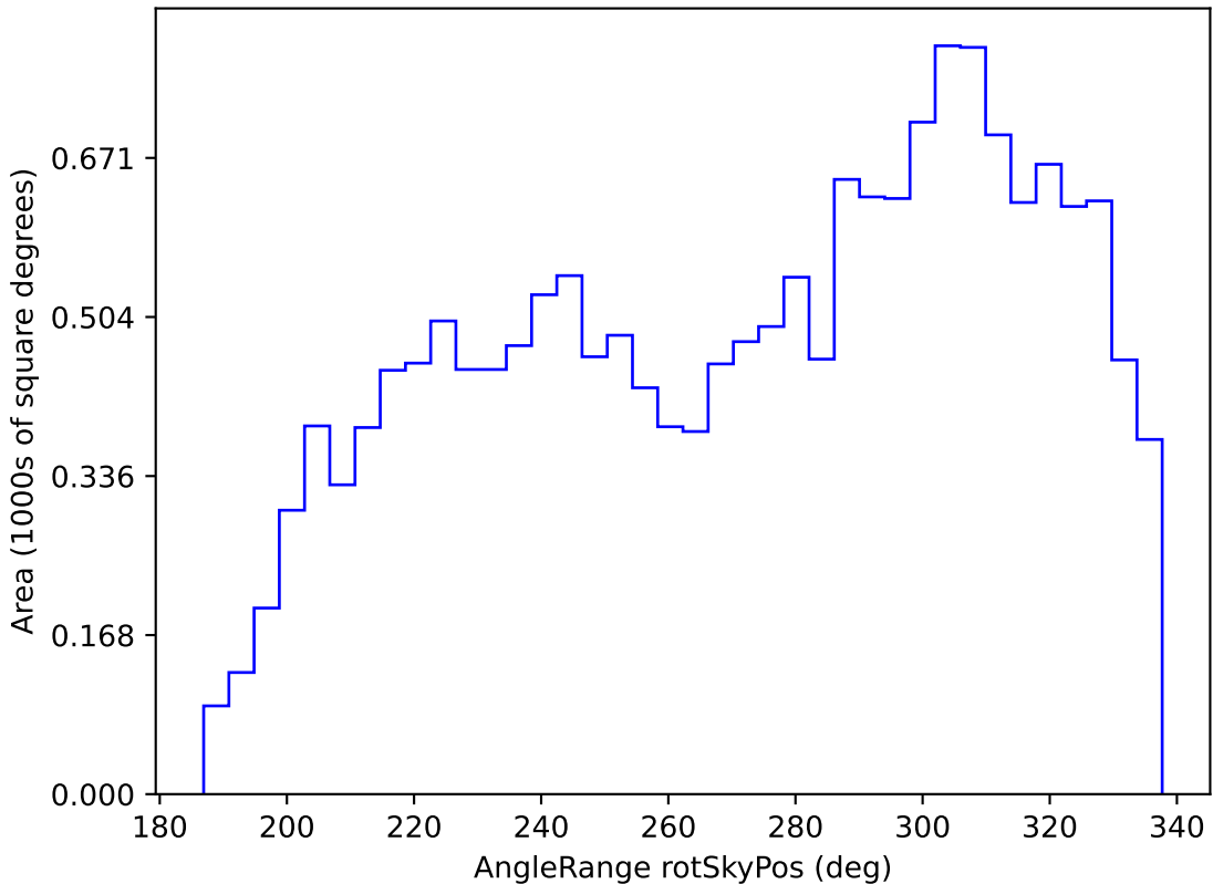
noroll_mjdp60_v3.4_10yrs WFD y band: AngleRange rotSkyPos
