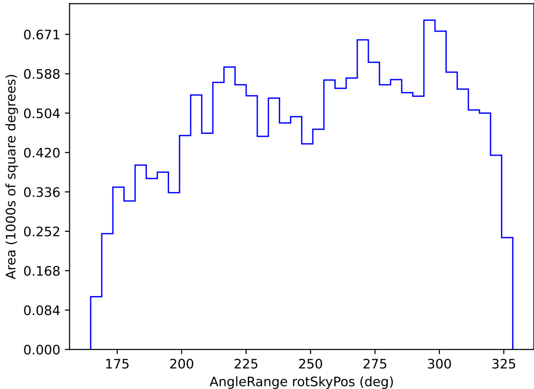
noroll_mjdp60_v3.4_10yrs WFD u band: AngleRange rotSkyPos
