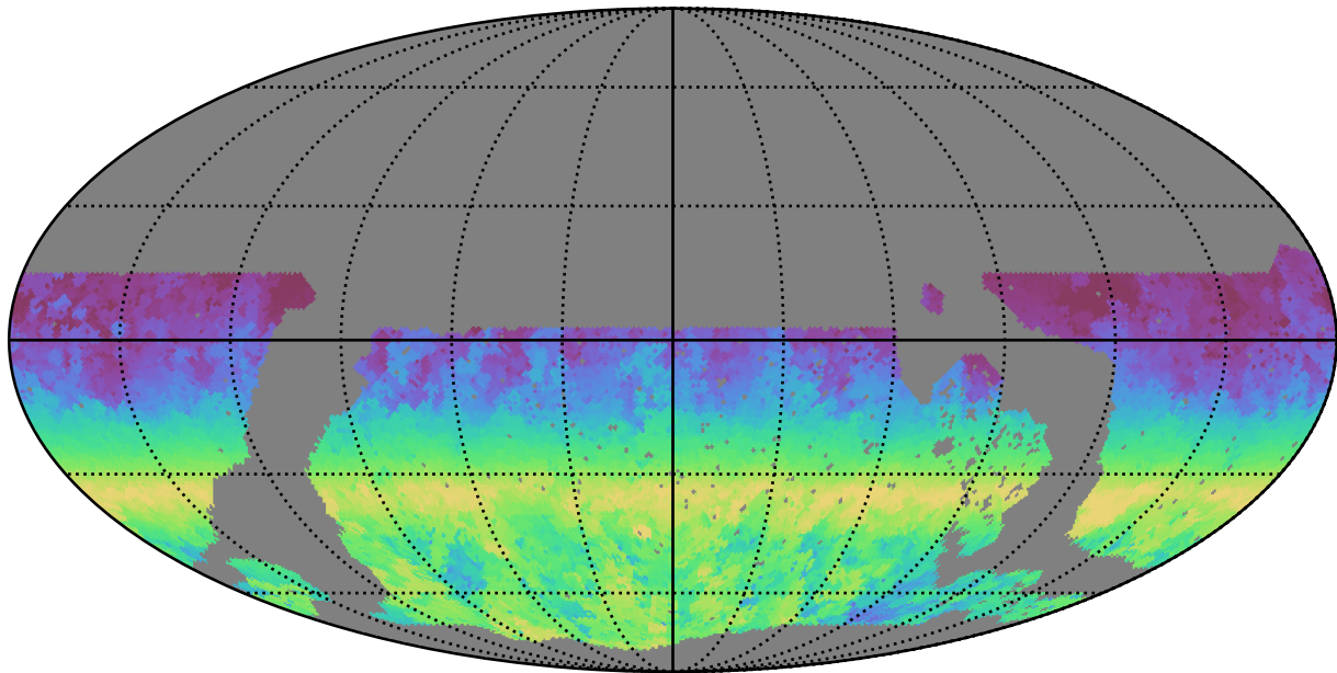
noroll_mjdp60_v3.4_10yrs WFD r band: AngleRange rotSkyPos
