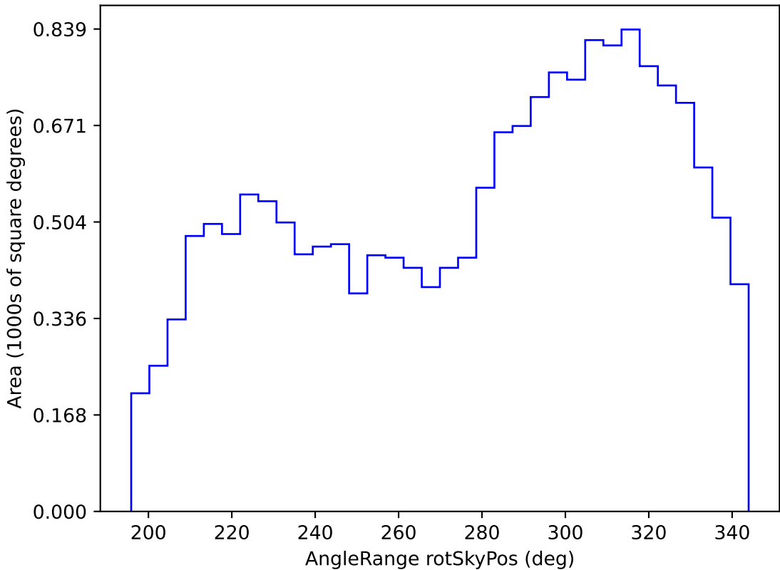
noroll_mjdp60_v3.4_10yrs WFD r band: AngleRange rotSkyPos
