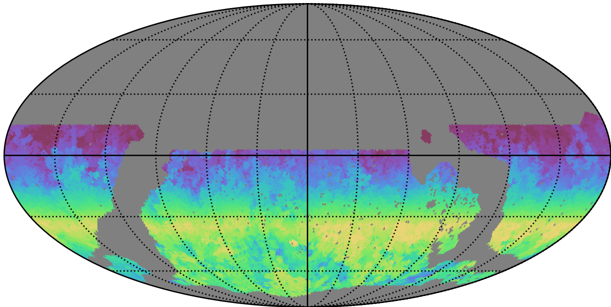
noroll_mjdp60_v3.4_10yrs WFD i band: AngleRange rotSkyPos
