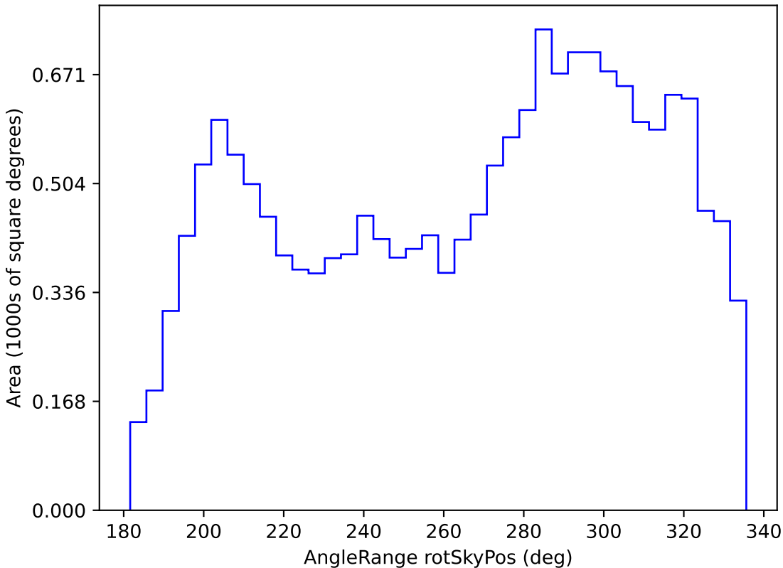
noroll_mjdp60_v3.4_10yrs WFD g band: AngleRange rotSkyPos
