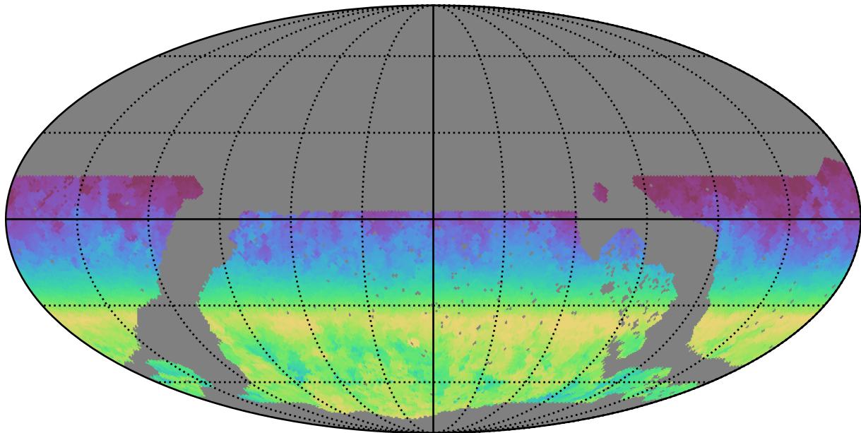
noroll_mjdp60_v3.4_10yrs WFD all bands: AngleRange rotSkyPos
