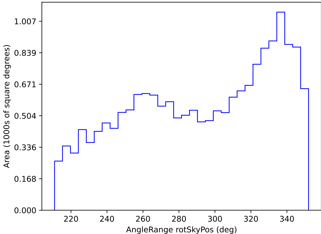
noroll_mjdp60_v3.4_10yrs WFD all bands: AngleRange rotSkyPos
