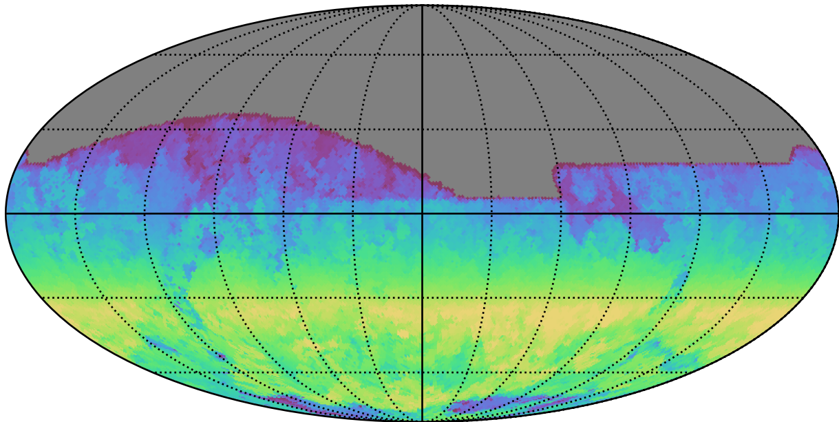
noroll_mjdp60_v3.4_10yrs All sky z band: AngleRange rotSkyPos
