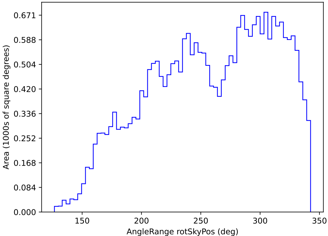
noroll_mjdp60_v3.4_10yrs All sky z band: AngleRange rotSkyPos
