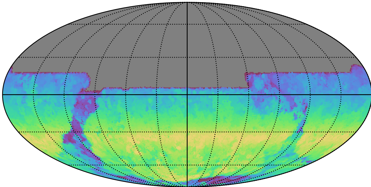
noroll_mjdp60_v3.4_10yrs All sky y band: AngleRange rotSkyPos
