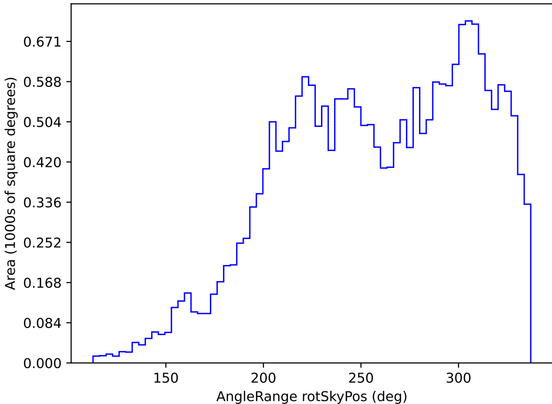
noroll_mjdp60_v3.4_10yrs All sky y band: AngleRange rotSkyPos
