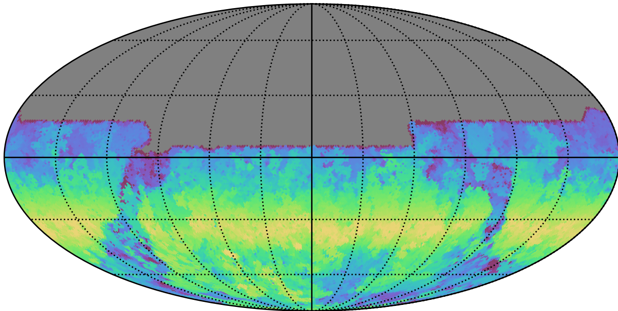
noroll_mjdp60_v3.4_10yrs All sky u band: AngleRange rotSkyPos
